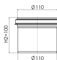
Gully Bottom outlet Ø110
