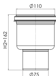
Gully Bottom outlet Ø75
