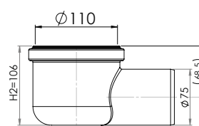
Gully Side outlet Ø75
