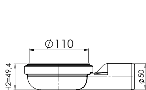
Gully, low built Side outlet Ø50
