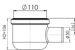
Gully Side outlet Ø50
