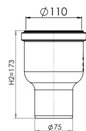
Gully Bottom outlet Ø75
